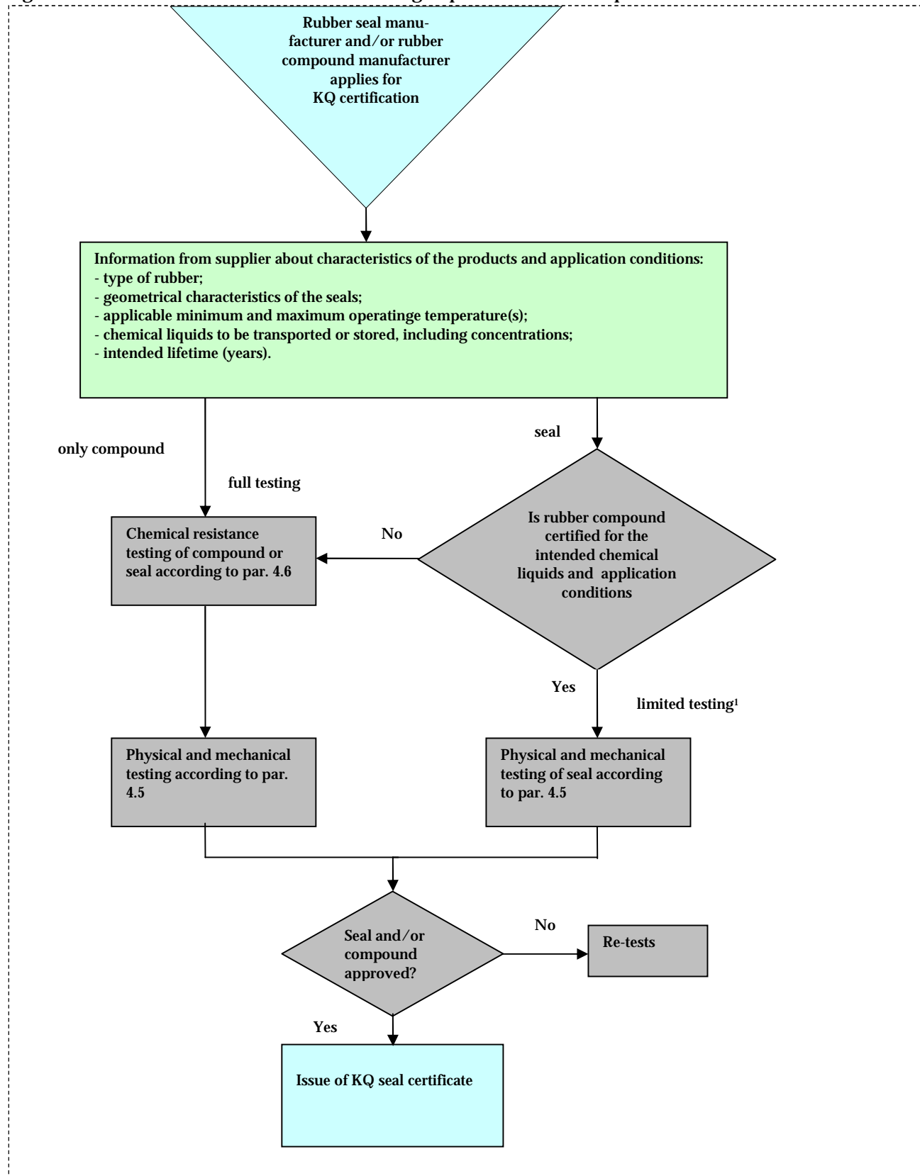
Figure 1: Flow chart of chemical resistance testing as part of certification process
